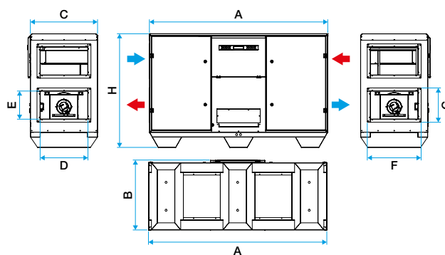
Dimensions VEX500
