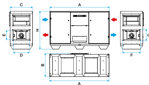
Dimensions VEX500
