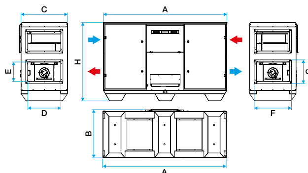
Dimensions VEX500
