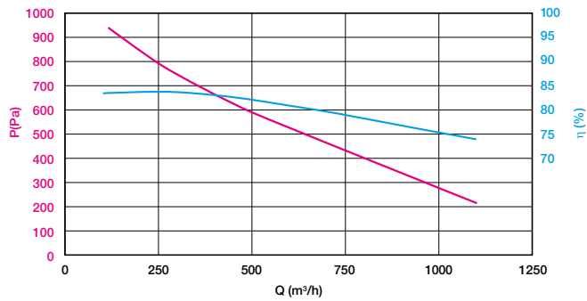
Aeraulic characteristics VEX720T
